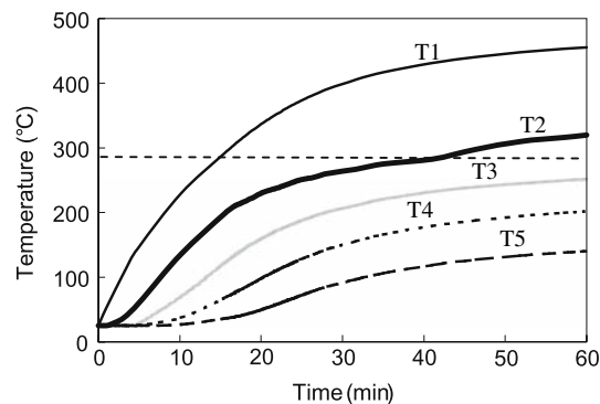
Fig. 8 Temperature of paulownia wood by FEM analysis
