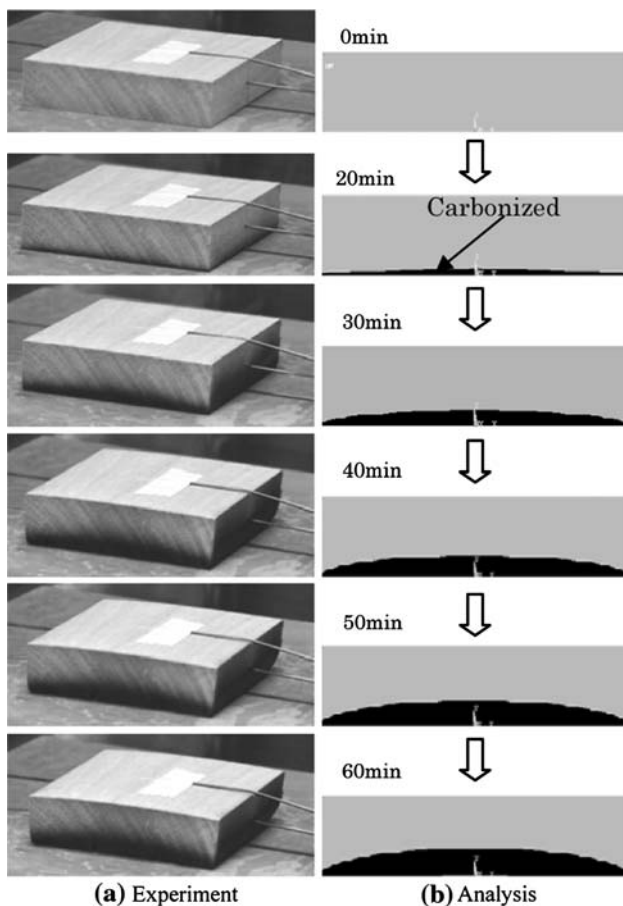
Fig. 7 Result of the heating experiment and FEM analysis of paulownia wood
