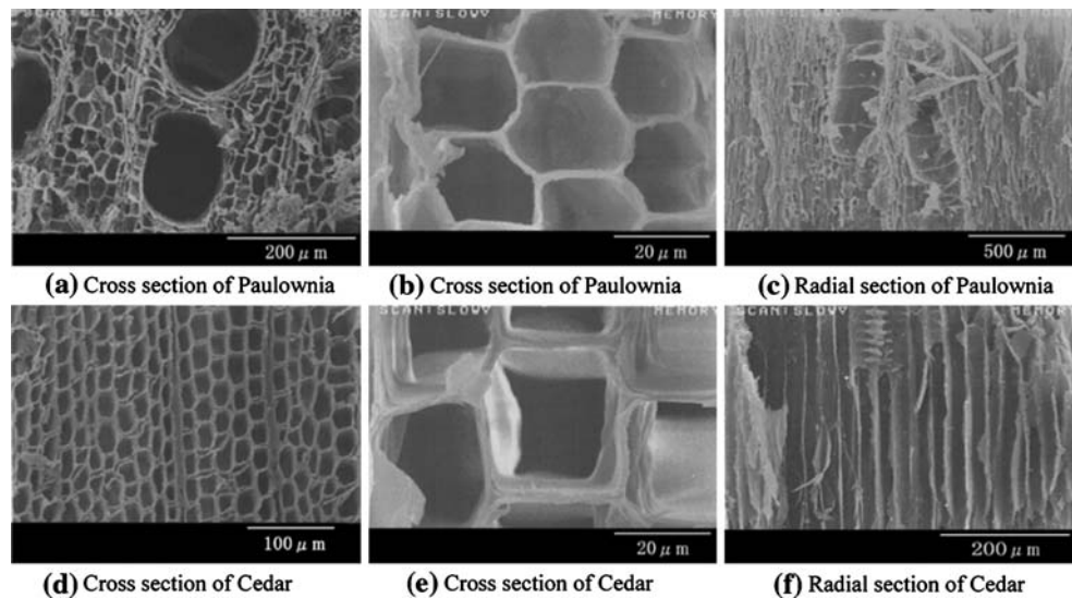
Fig. 4 SEM micrographs of the wood
