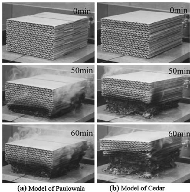
Fig. 11 The result of heating the model
