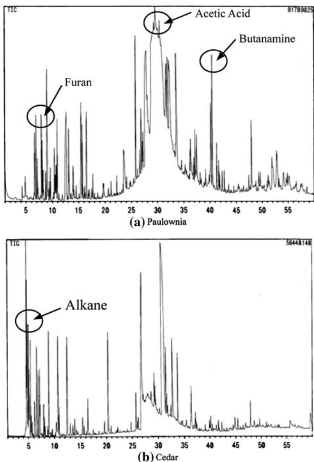
Fig. 9 Gas chromatography analysis upon heating the wood
