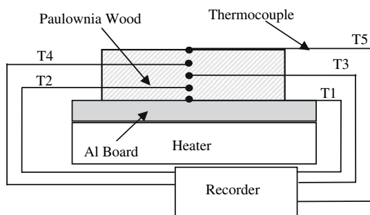
Fig. 5 Appearance of heating experiment
