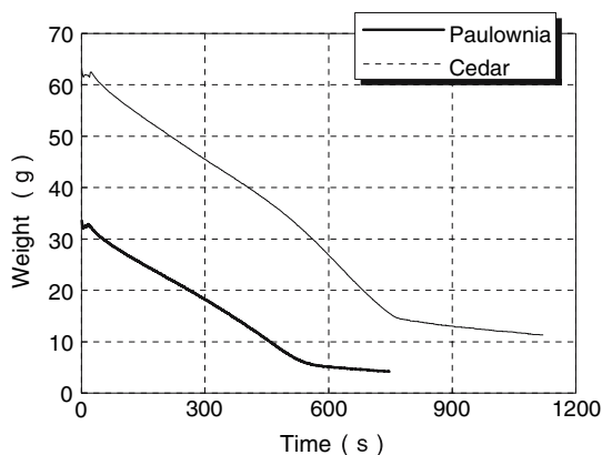
Fig. 2 Time–weight curves at 50 \text{ kW m}^{-2} of heat flux
