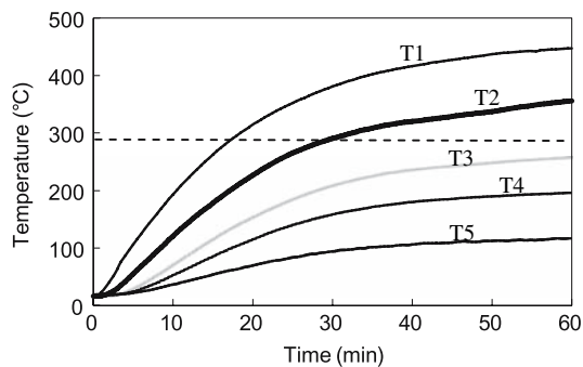
Fig. 6 Temperature of heating experiment
