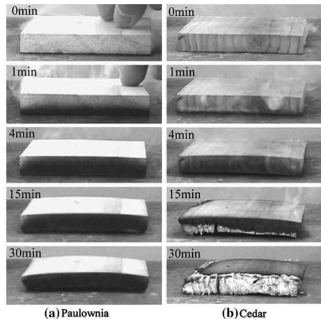
Fig. 1 Appearance of heating wood board
